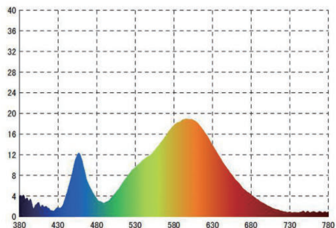
Absolute spectrum
