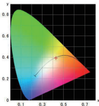
Chromaticity diagram
