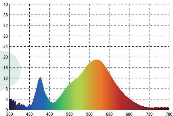
Absolute spectrum
