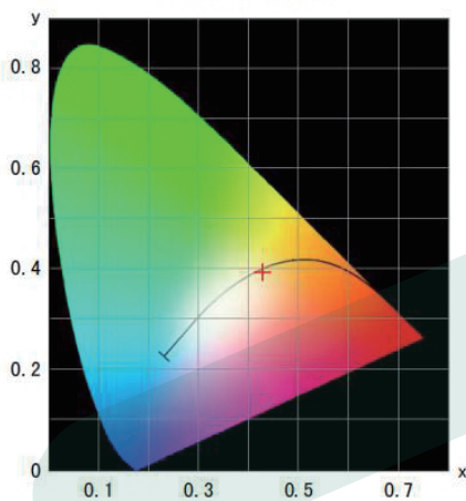
Chromaticity diagram
